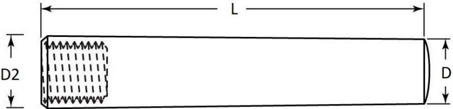
Extractable Type (Internal Thread)
